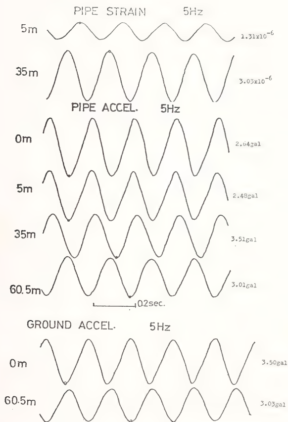
Fig. 3 Measured Sinusoidal Waves
